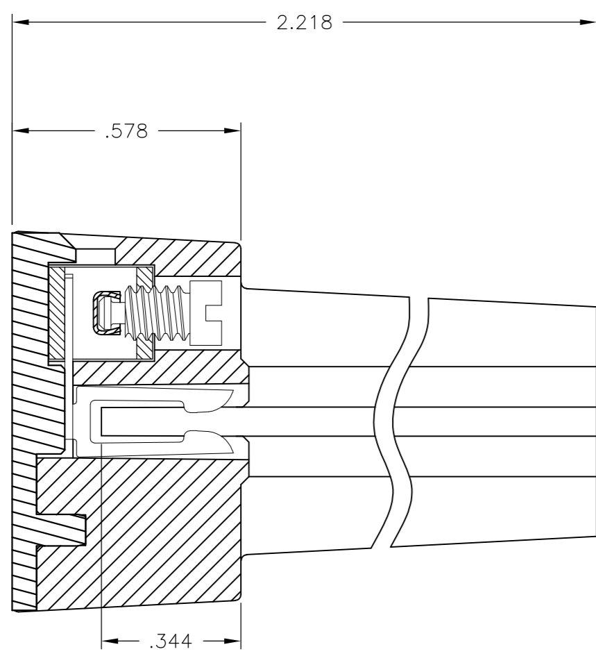
MATING BOARD DEPTH SECTION A-A
