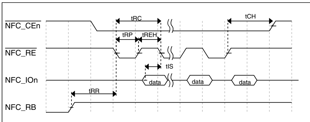
Figure 38. Read data latch cycle timing in Fast mode and EDO mode
