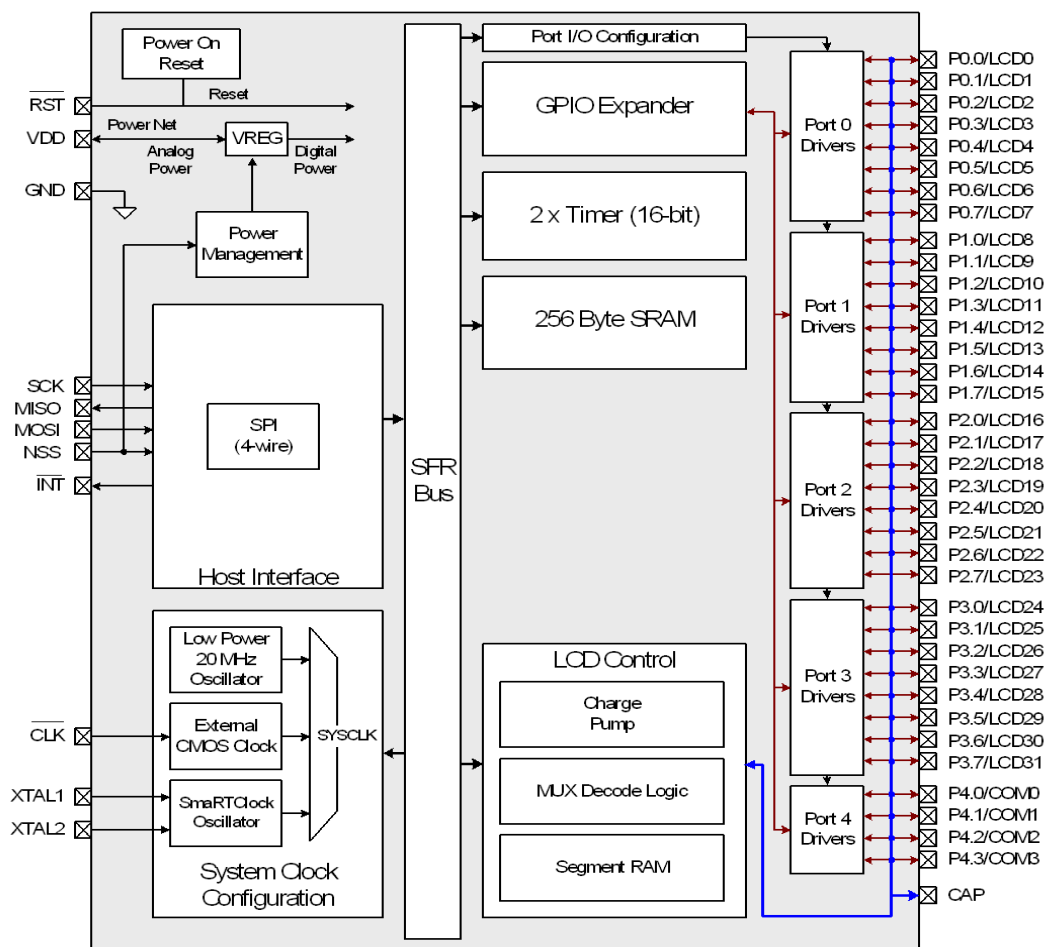
Figure 1.1. CP2400 Block Diagram
