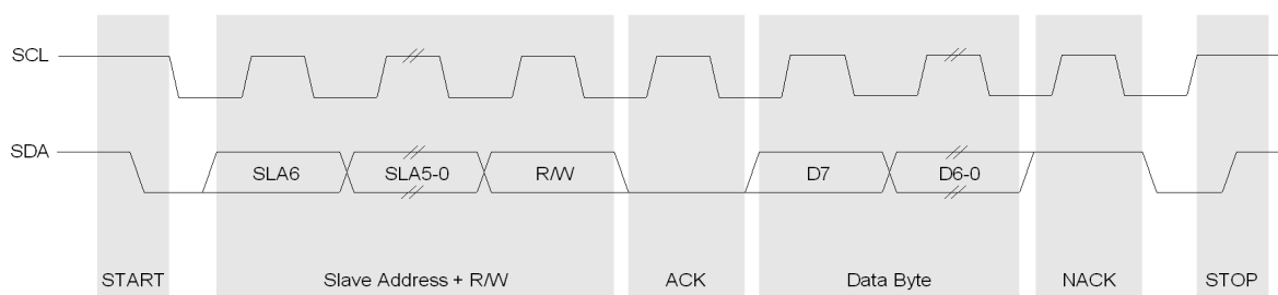
Figure 15.2. SMBus Transaction
