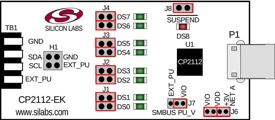
Figure 6. CP2112 Evaluation Board with Default Shorting Blocks Installed
