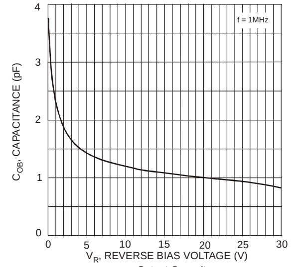
Fig.10 Output Capacitance
