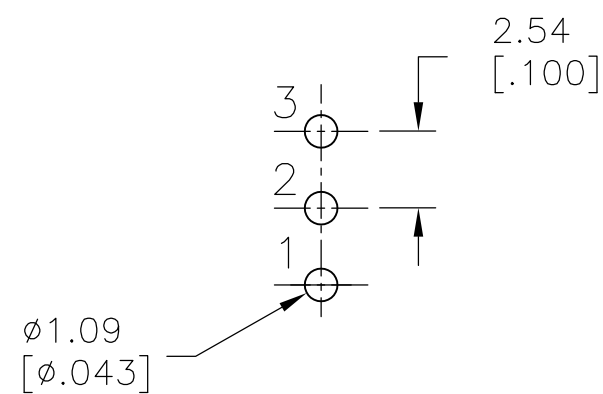
P.C. MOUNTING
