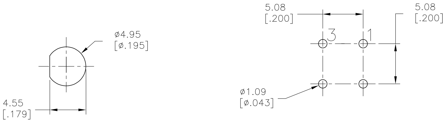
P.C. MOUNTING
