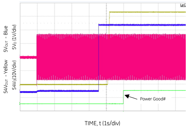
Figure 14. Turn-ON at full load V_{IN} = 230V_{AC} .
