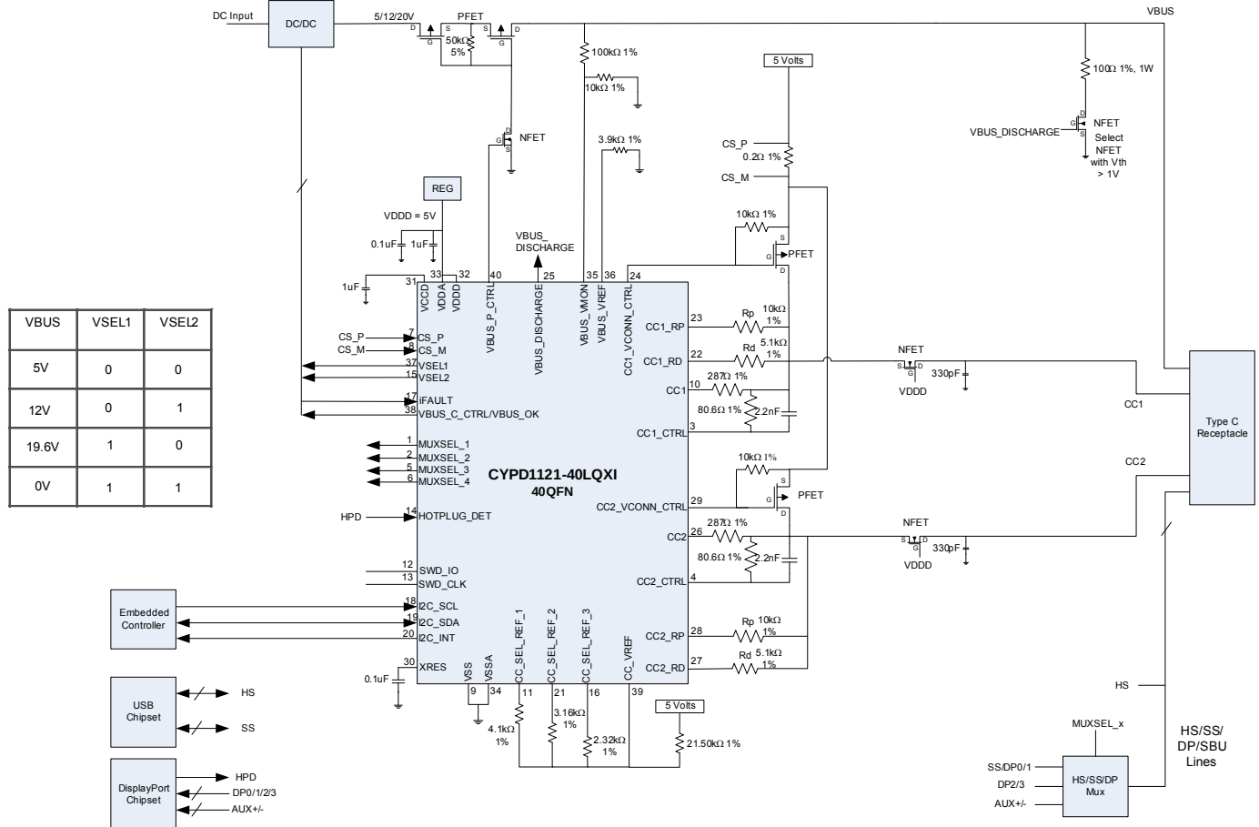
Figure 11. Monitor Application Block Diagram
