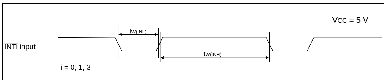
Figure 5.30 External Interrupt \overline{\text{INTi}} Input Timing Diagram when V_{CC} = 5\text{ V}
