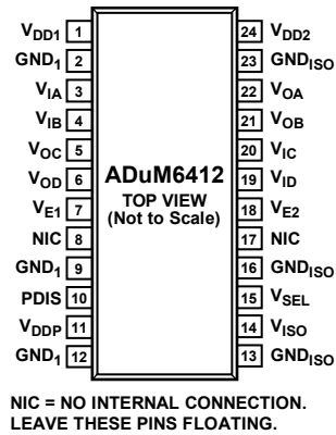
Figure 5. ADuM6412 Pin Configuration
