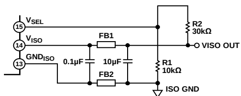
Figure 31. V_{ISO} Bias and Bypass Components
