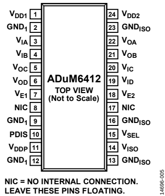
Figure 5. ADuM6412 Pin Configuration
