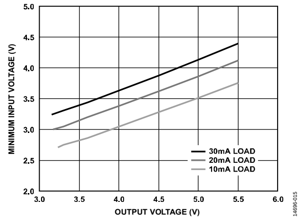
Figure 15. Relationship Between Output Voltage and Required Input Voltage, Under Load, to Maintain >80% Duty Factor in the PWM
