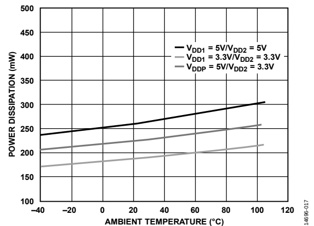
Figure 17. Power Dissipation vs. Ambient Temperature with a 20 mA Load
