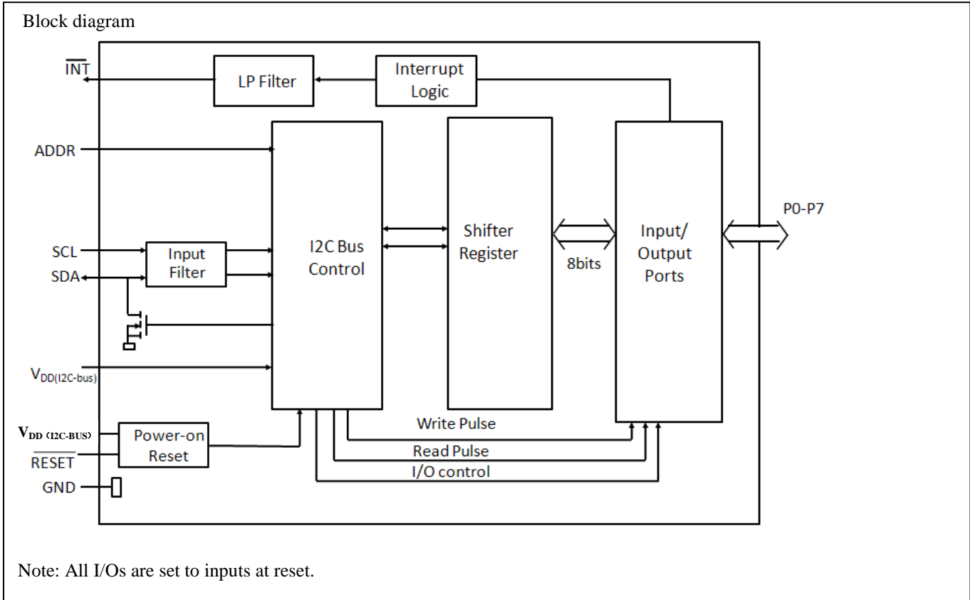
Fig 5: Block diagram
