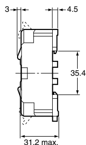
Terminal Arrangement (Top View)
