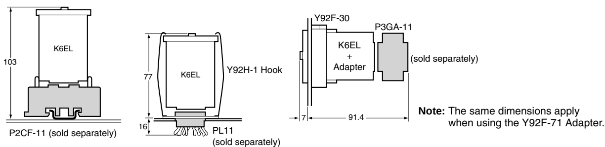
P2CF-11 Front Connecting Socket
