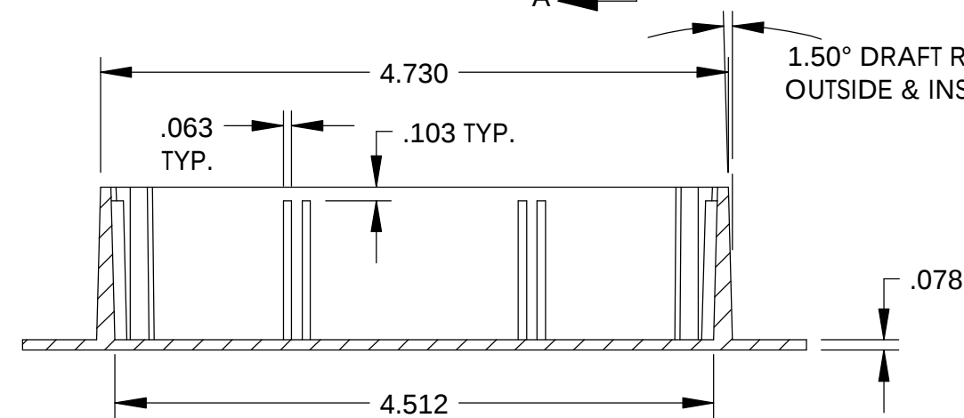
SECTION B-B
