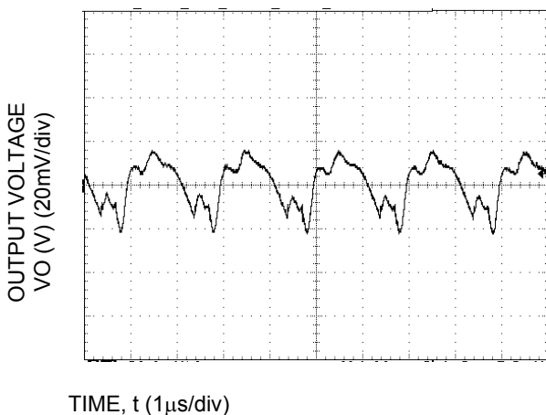
Fig-35. Typical output ripple and noise (CO=2x47uF ceramic, VIN = 12V, Io = Io,max, ).
