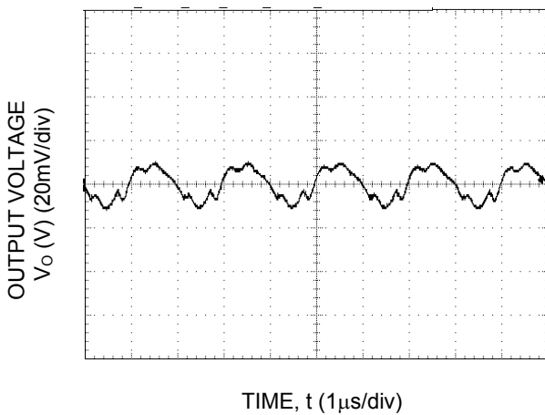
Fig-23. Typical output ripple and noise (CO=2x47uF ceramic, VIN = 12V, Io = Io,max, ).
