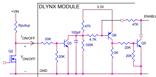
Fig-3: Circuit configuration for using positive On/Off logic.
