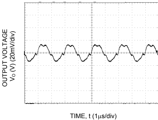
Fig-17. Typical output ripple and noise (CO=2x47uF ceramic, VIN = 12V, I o = I o,max ).
