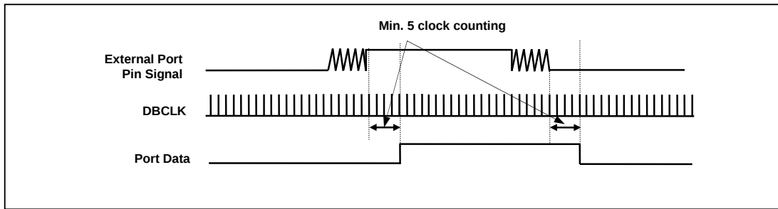
Figure 2.4 Debounce Function
