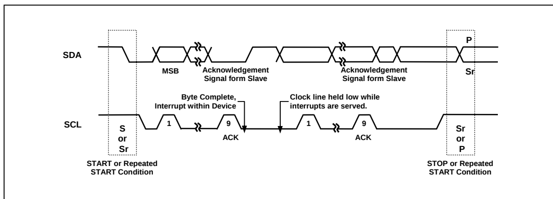
Figure 4.30 Data Transfer on the I2C-Bus
