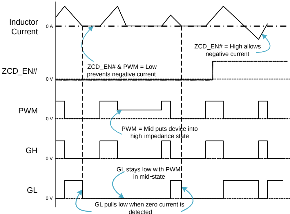
Figure 9. Zero Cross Detect Functionality
