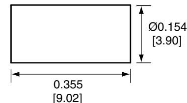
CRIMP RING
