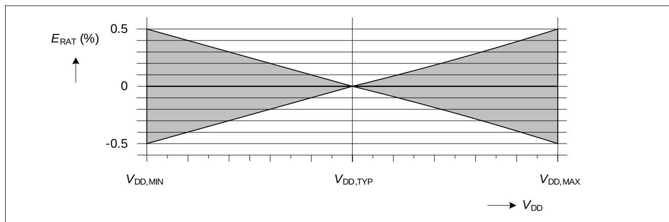
Figure 4 Ratiometric error
