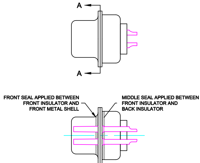
DETAIL A-A SHOWN FOR REFERENCE ONLY
