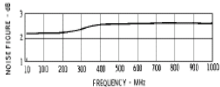
Noise Figure
