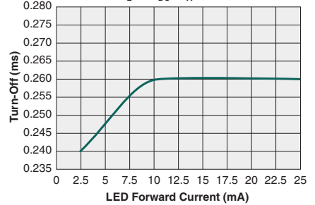
Typical Turn-Off vs. LED Forward Current ( I_L=1\text{A}_{DC} , T_A=25^\circ\text{C} )
