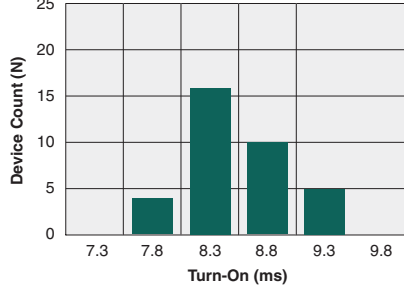
Typical Turn-On Time (N=35, I_F=20\text{mA} , I_L=1\text{A}_{DC} , T_A=25^\circ\text{C} )
