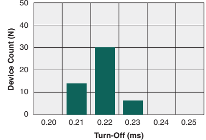
Typical Turn-Off Time (N=50, I_F=20\text{mA} , I_L=1\text{A}_{DC} , T_A=25^\circ\text{C} )
