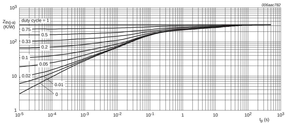
Fig 2. Transient thermal impedance from junction to ambient as a function of pulse duration for PDA114EE (SOT416); typical values
