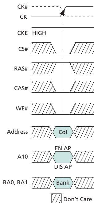
Figure 18: WRITE Command
