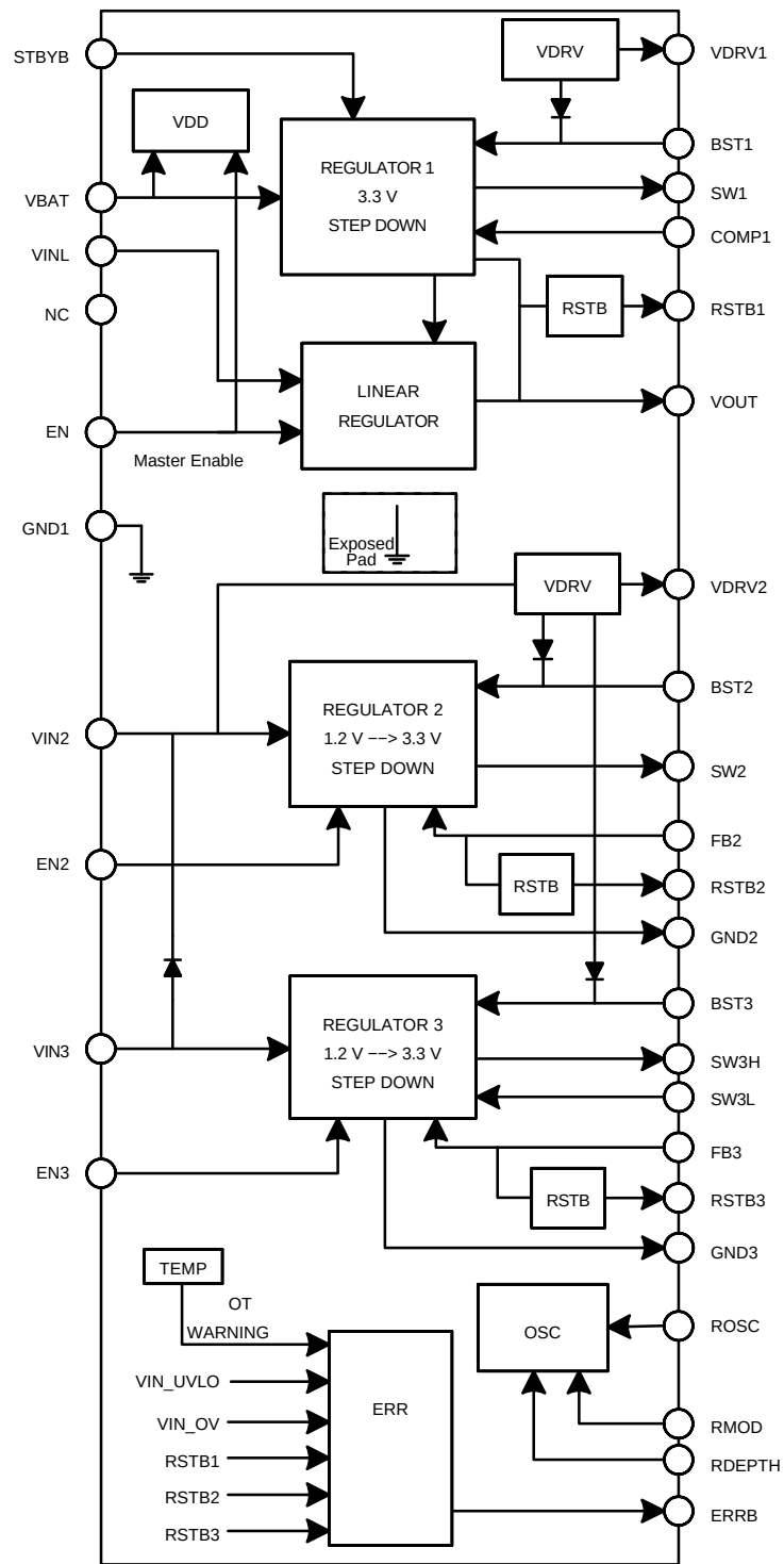
Figure 2. NCV97310 Block Diagram – 3.3 V Version
