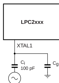
Fig 27. Slave mode operation of the on-chip oscillator
