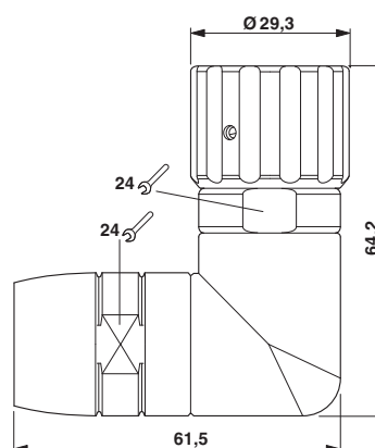
Dimensional drawing
