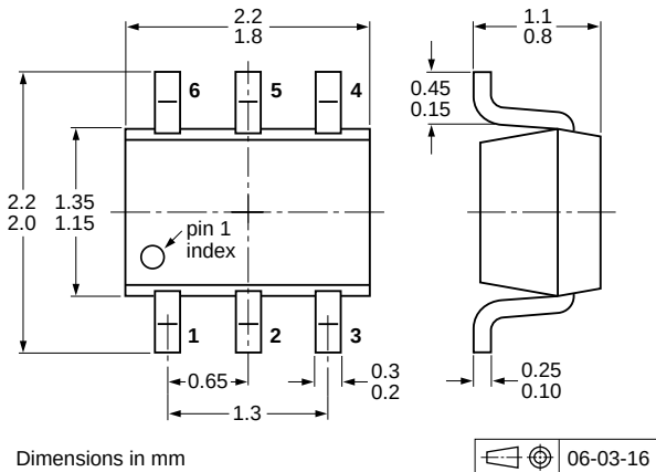
Fig 11. Package outline PUMH13 (SOT363)
