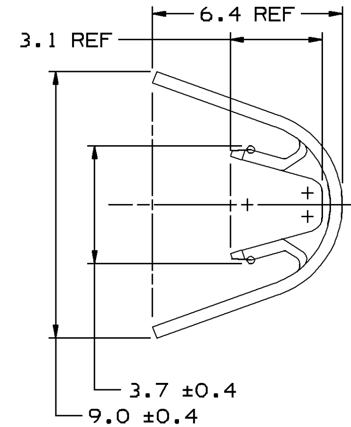
CARRIER STRIP VIEW SCALE 2:1
