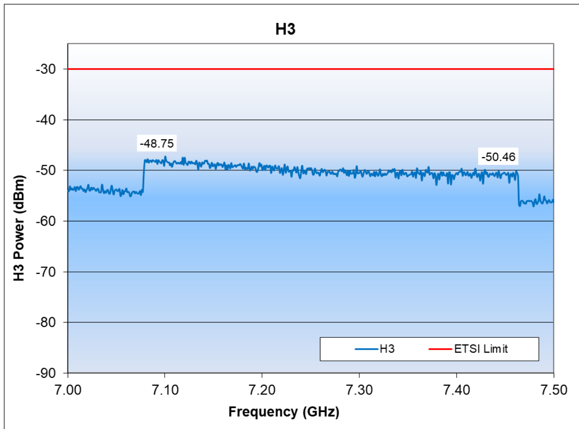
Figure 23. Conducted H3 spurious
