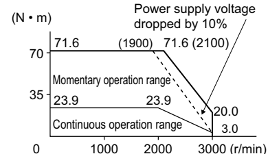
R88M-K5K020(H/T)-□ (5 kW)
