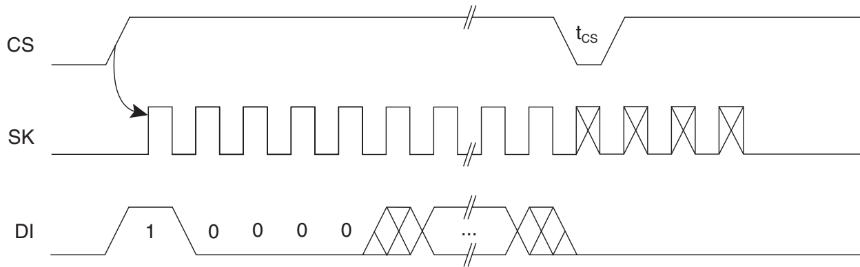
Figure 5. EWDS Timing
