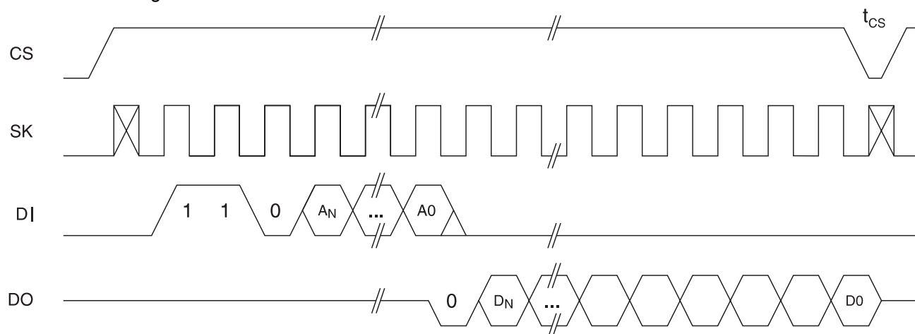
Figure 3. READ Timing
