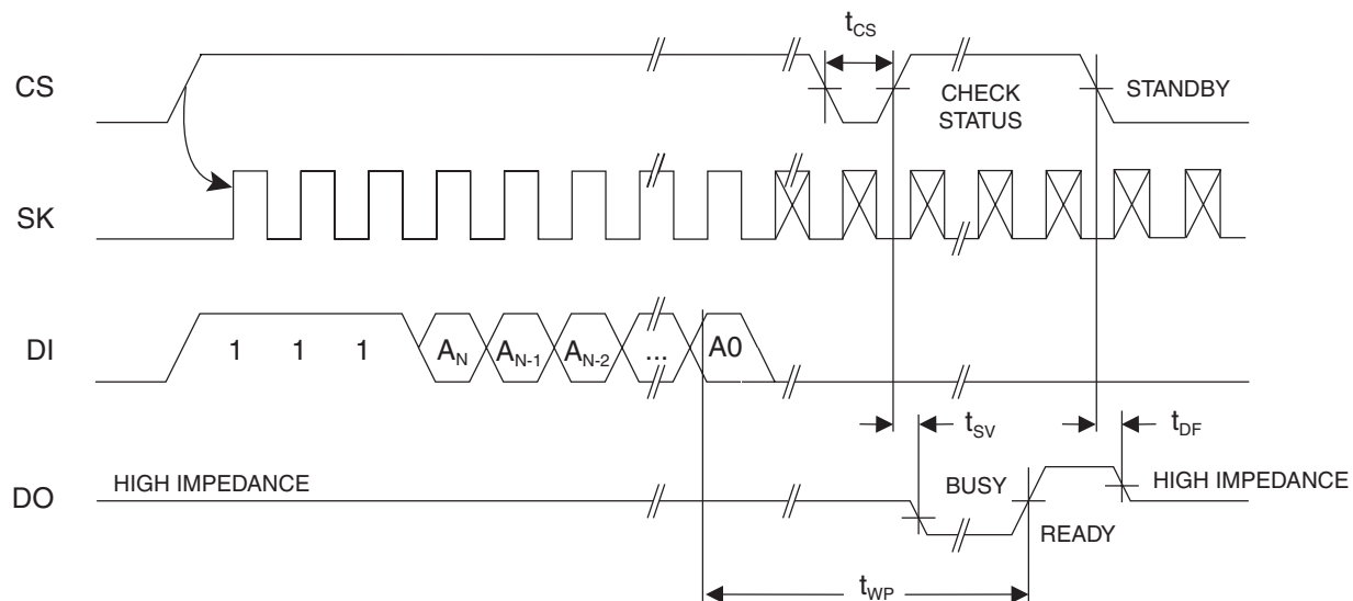
Figure 8. ERASE Timing
