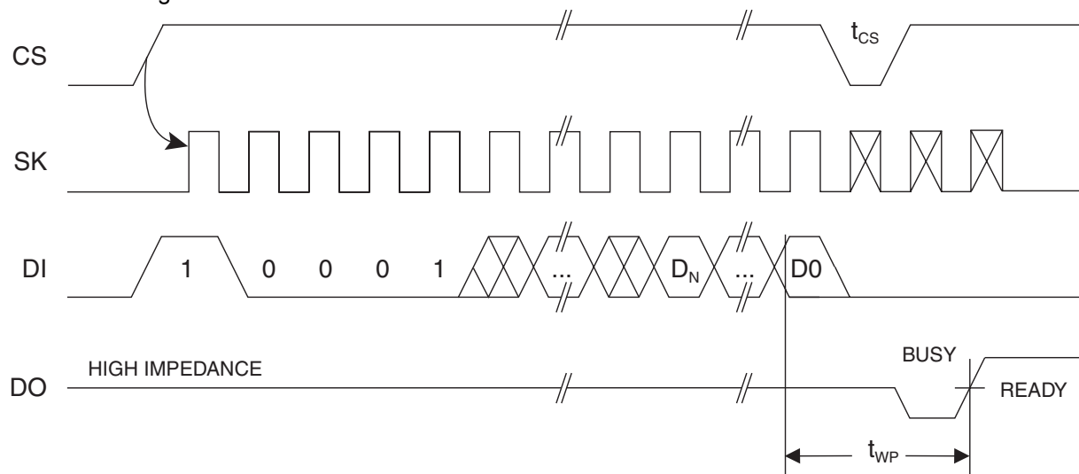
Figure 7. WRAL Timing (1)
