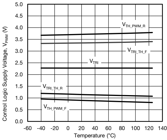
Fig. 19 - PWM Threshold vs. Temperature (SiC620R)
