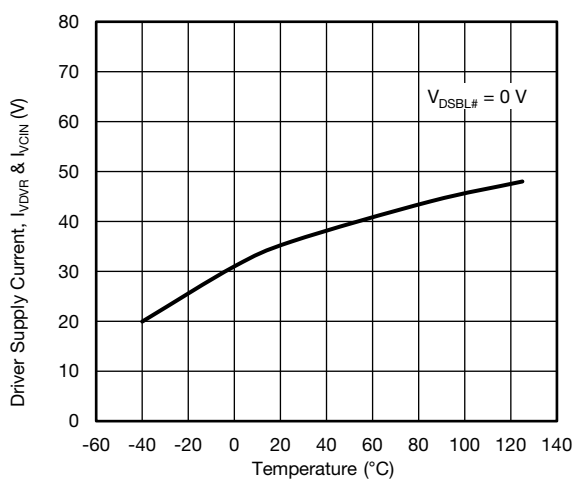
Fig. 27 - Driver Shutdown Current vs. Temperature
