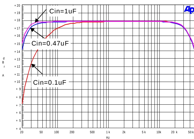
5. Frequency Response
