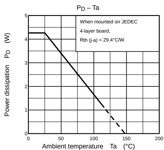
TC78B042FTG (QFN32)
