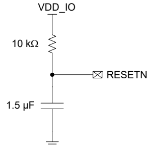
Figure 5. Reset Connection
