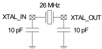
Figure 4. Crystal Connection
