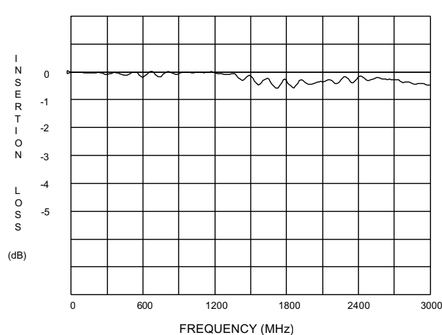
INSERTION LOSS (TYPICAL)
