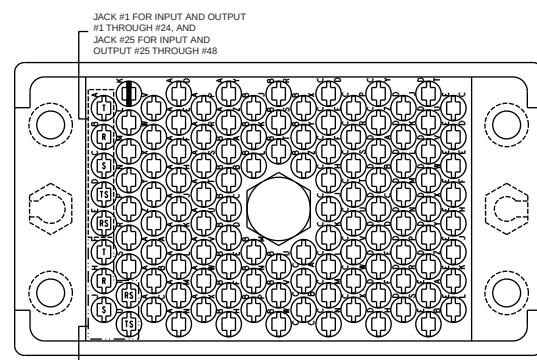
JACK #1 FOR INPUT AND OUTPUT #13 THROUGH #24, AND JACK #25 FOR INPUT AND OUTPUT #25 THROUGH #48
