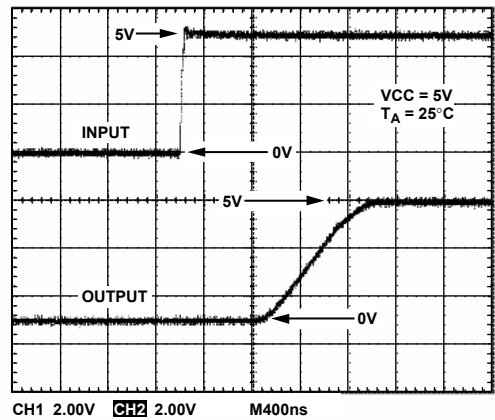
Figure 10. Transient Response—Rising
