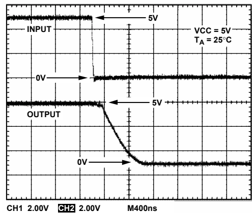
Figure 11. Transient Response—Falling
