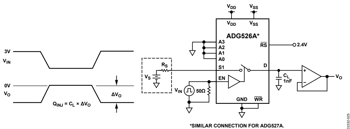
Figure 25. Charge Injection
