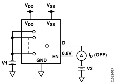
Figure 17. I_D (Off)
