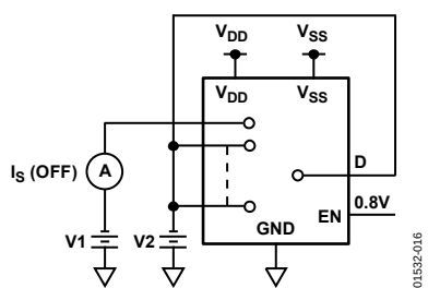
Figure 16. I_S (Off)
