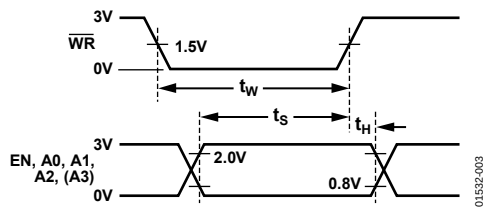
Figure 13. Timing Sequence
