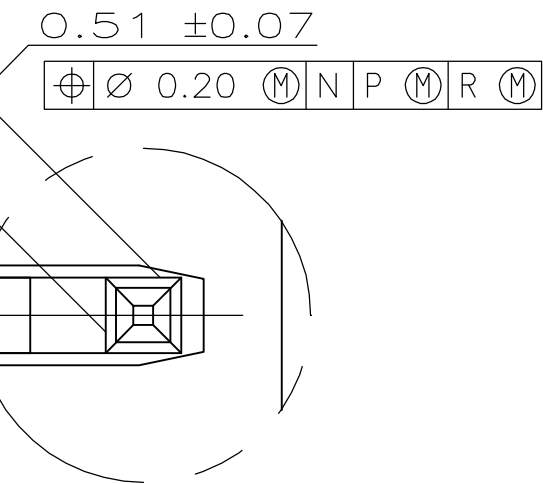
DETAIL Z SCALE 20:1
