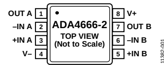
Figure 1. 8-Lead MSOP
