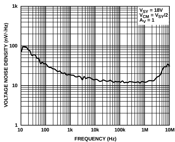
Figure 59. Voltage Noise Density vs. Frequency
