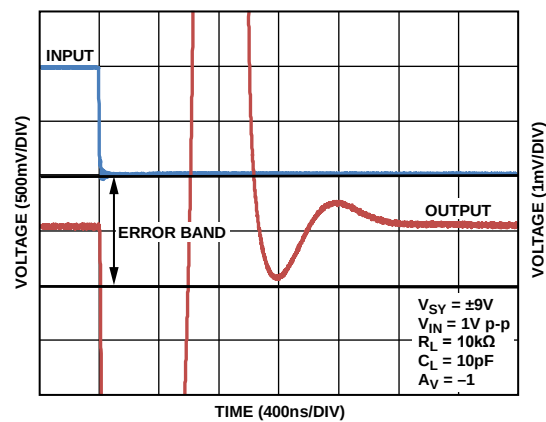
Figure 58. Negative Settling Time to 0.1%
