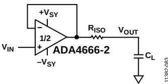
Figure 83. Stability Compensation with Isolating Resistor, R_{ISO}
