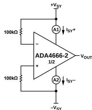
Figure 75. Comparator A
