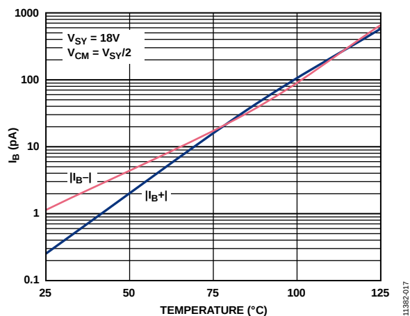
Figure 21. Input Bias Current vs. Temperature
