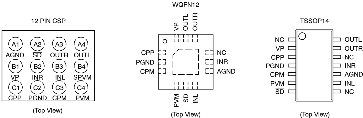
Figure 2. Pin Configurations
