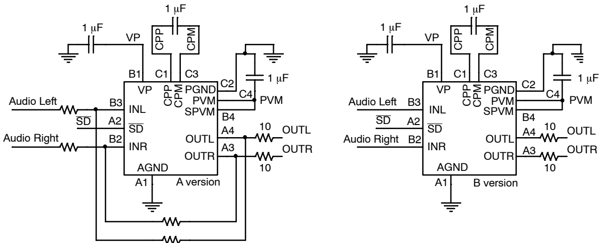
Figure 1. Application Schematics
