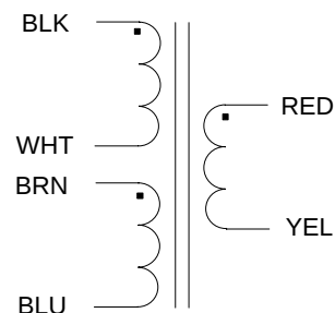
SCHEMATIC
