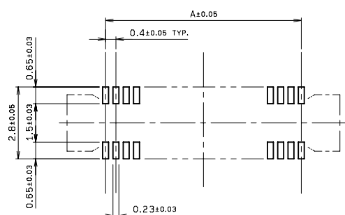
MOUNTING LAYOUT
